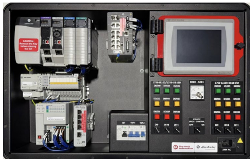
ABT-TDENET-B-CE (EtherNet/IP Networking Workstation)
